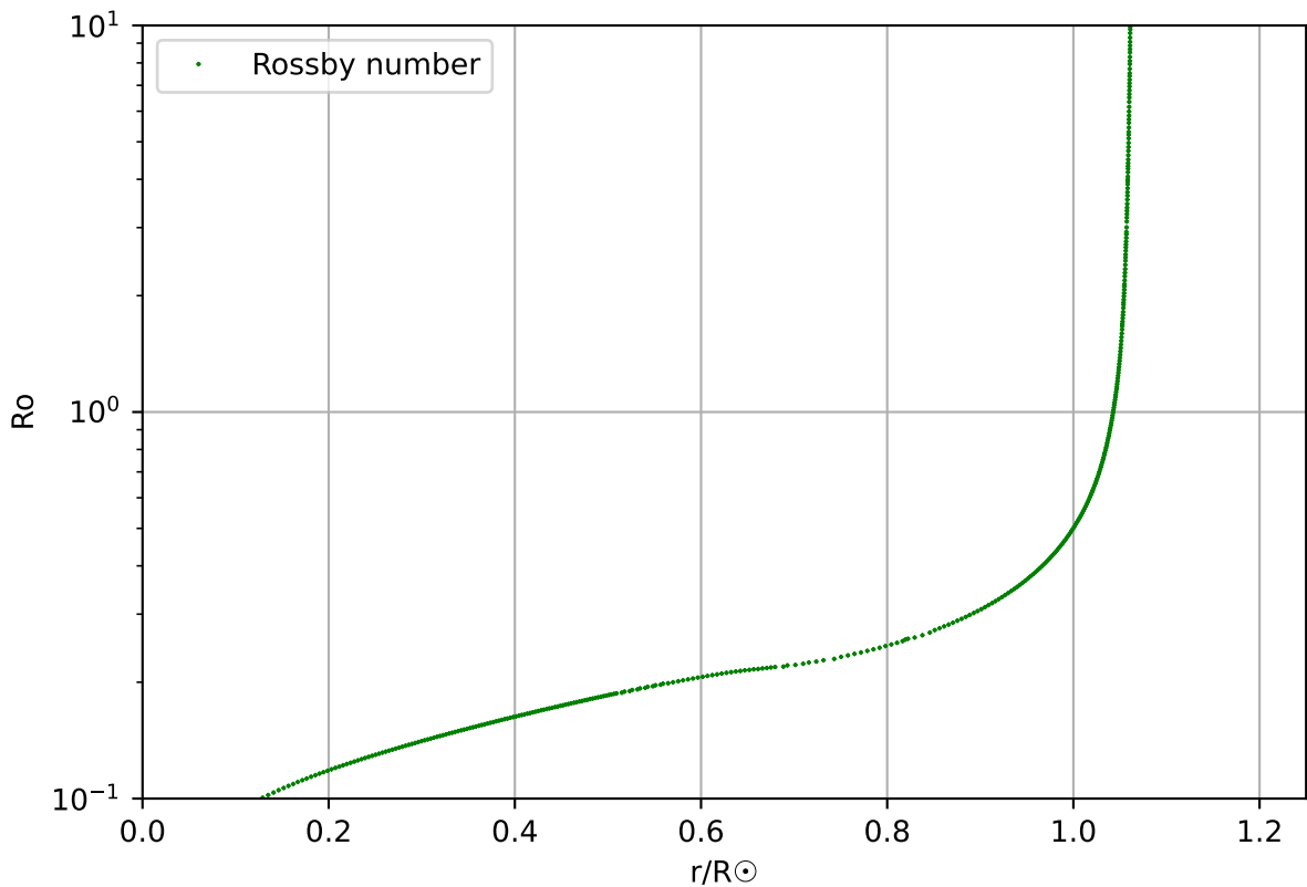
Rossby number, profile 109, age 2.05 \times 10^7
